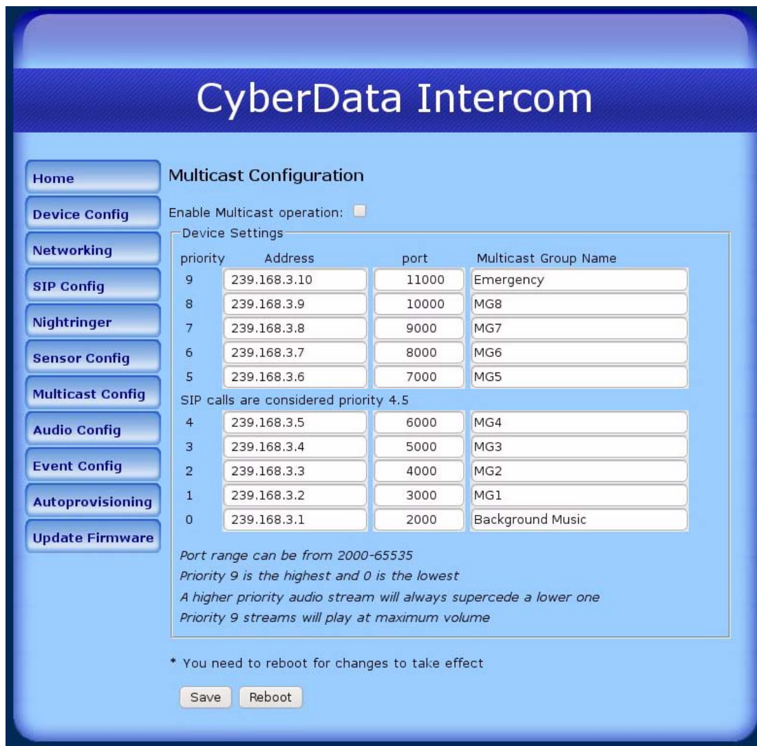
Figure 6. Multicast Configuration Page
