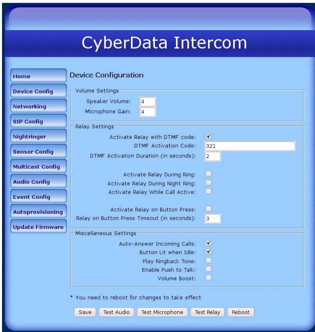
Figure 3. Device Configuration Page
