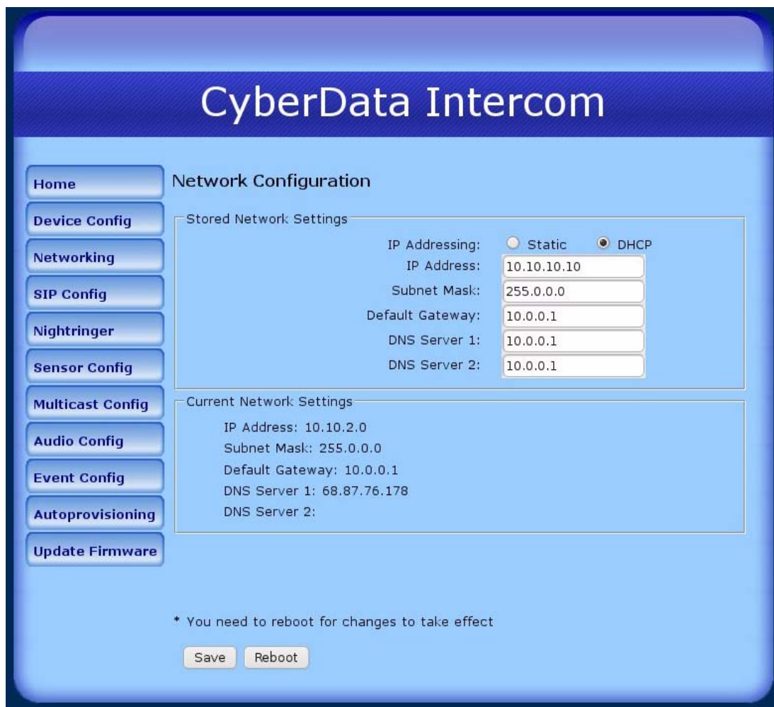
Figure 4. Network Configuration Page
